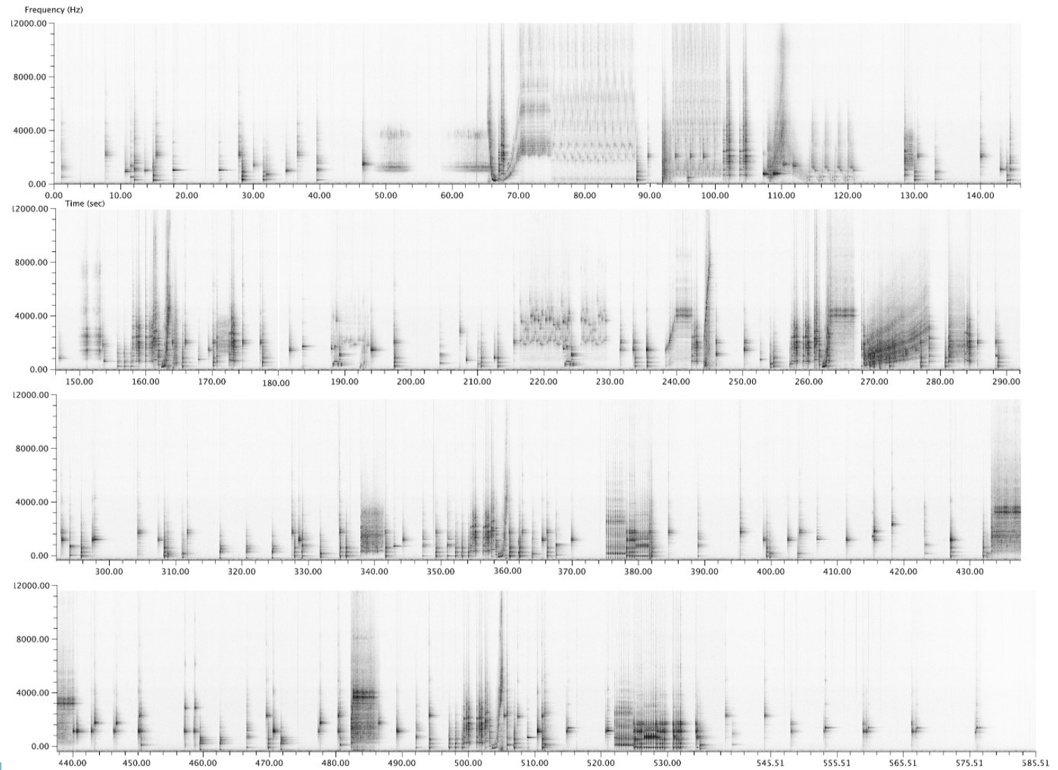
Figure 4.20 – Spectrogram of Water Music
